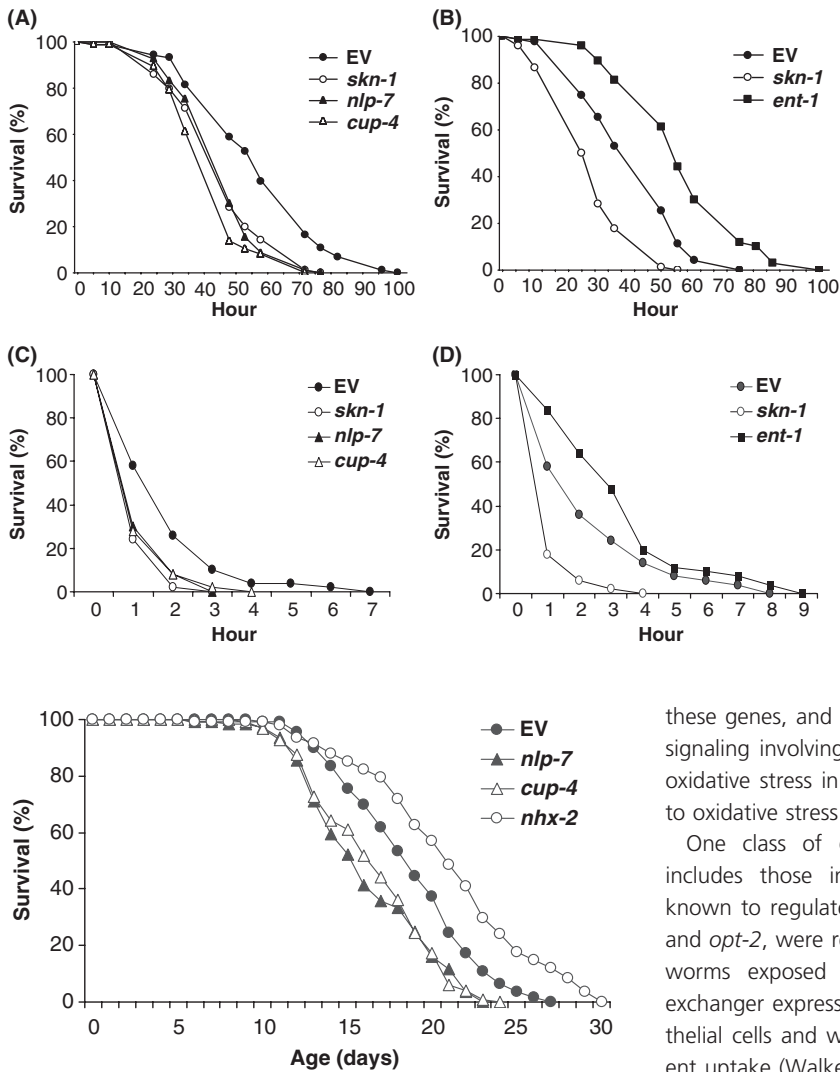
Fig. 3 Lifespan of N2 fed with dsRNA of skn-1 -dependent oxidative-stress genes. Animals were scored at 20 °C from egg hatch until all worms were dead. Each longevity assay was replicated and the average of two assays was plotted. Mean lifespan of nlp-7 RNAi ( 15.2 \pm 0.6 SEM) and cup-4 RNAi ( 15.6 \pm 0.6 SEM) was significantly reduced ( P = 0.004 and 0.001 for nlp-7 RNAi and P = 0.014 and 0.003 for cup-4 RNAi) compared to control RNAi ( 17.7 \pm 0.5 SEM), while RNAi of nhx-2 increased ( P = 0.002 and 0.005 ) the mean lifespan ( 19.2 \pm 0.3 SEM). Means of duplicates are shown. EV: control empty vector.
