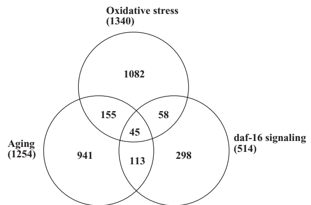
Fig. 1 Venn diagram of differential expression by oxidative stress, aging, and daf-16 . Number of overlapping genes in each comparison is greater than expected by chance ( P \ll 0.001 by Fisher's exact test). The representation factors of each comparison are 2.3 for oxidative stress and aging, 2.9 for oxidative stress and daf-16 , and 4.8 for aging and daf-16 . Lists of overlapping genes are provided as supporting information.
